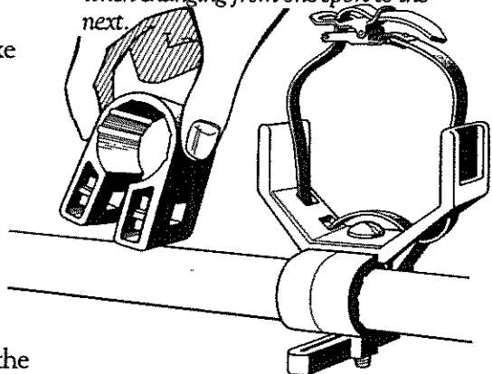
Snap-arounds, the heart of the Tran-Sport System, for easy on and off convenience of Yakima accessories without tools!
